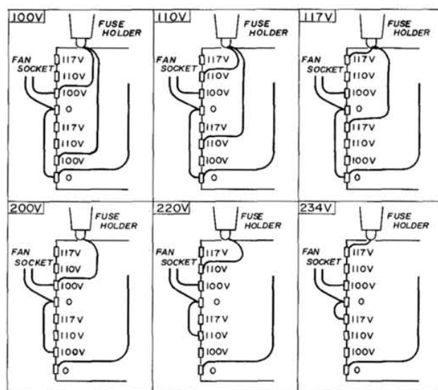
POWER TRANSFORMER CONNECTIONS
