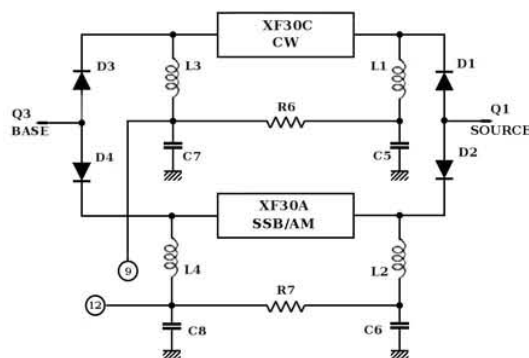
CW FILTER INSTALLATION DIAGRAM
