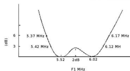
BANDPASS NETWORK CHARACTERISTICS
